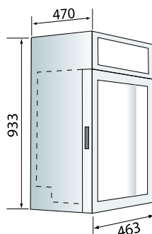
GLASS 84 +2°C / +10°C
