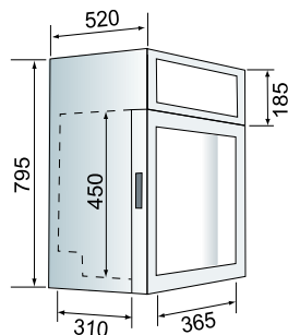
GLASS 54 +2°C / +10°C
