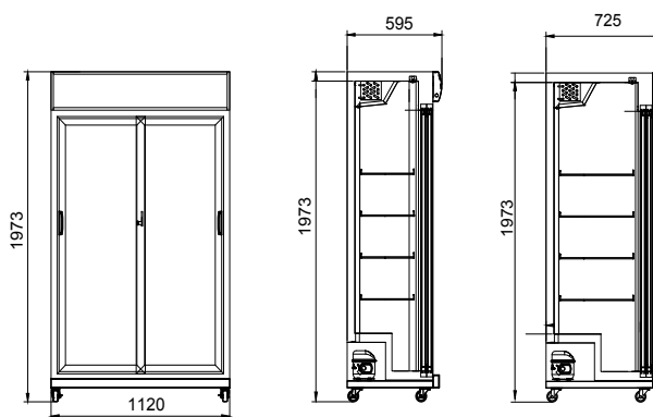
IDEAL-C 1002 Portes coulissantes
