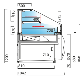
Semi-verticale libre-service
